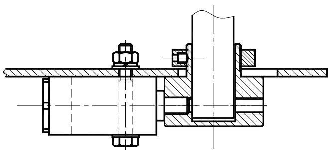
Fig. 1 Attacco filettato Threaded connection
