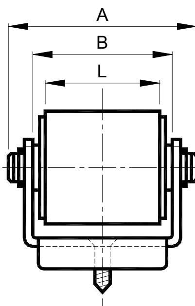
具保护层不锈钢滚轮 Rollerset in stainless steel with shields
